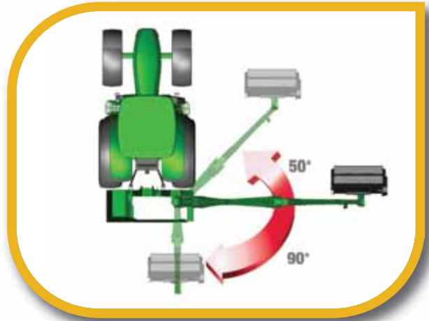
Rear Three Point Linkage Mounted Option
